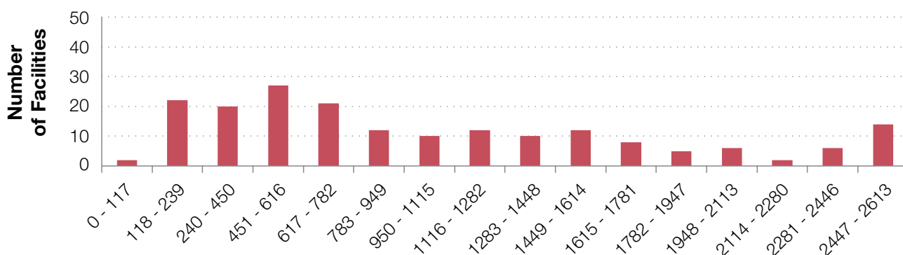
Figure 3.4. Energy intensities of Ontario sewage treatment facilities in 2011 in equivalent kilowatt hours per megalitre
