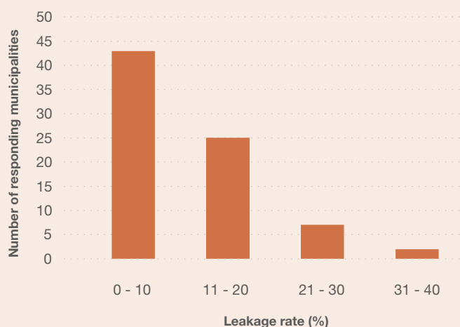
Figure 2.6. Ontario municipal water system leakage rates
