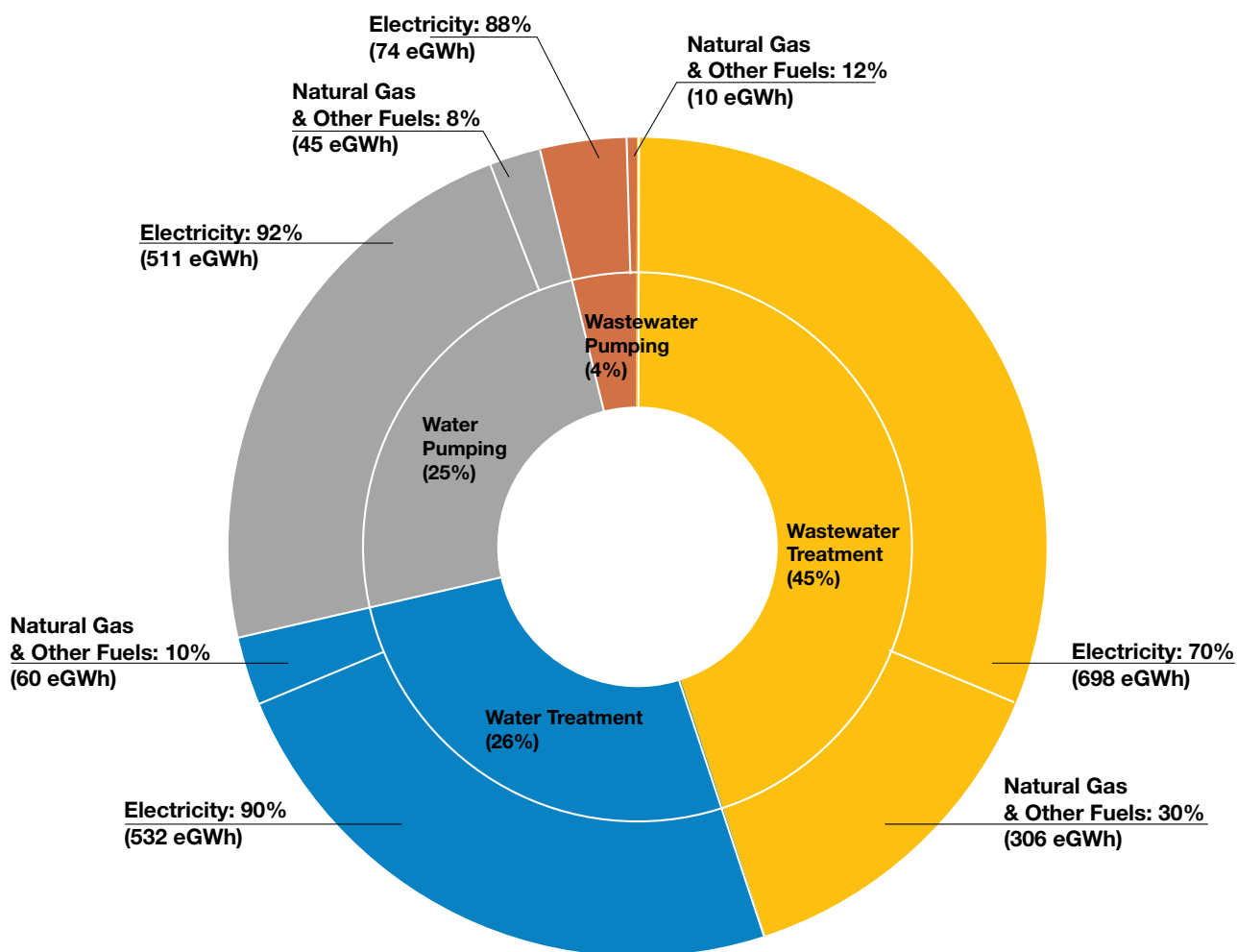
Figure 2.4. Ontario municipal water system electricity and natural gas consumption by facility type, in equivalent gigawatt hours (2011)
